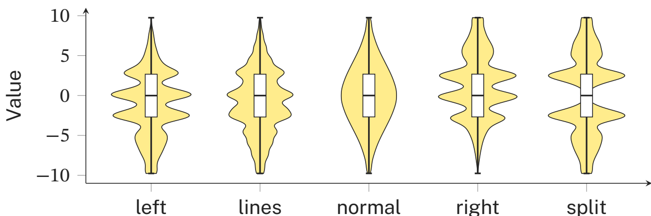
Figure 12. Five authentic teaching datasets from Matejka and Fitzmaurice, distributed through datasauRus . Each has 2,484 observations and nearly equal five-number summaries; the density shapes show what those summaries omit.
